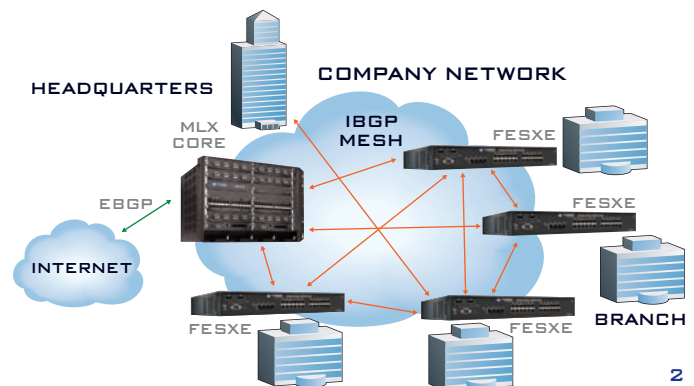
FIGURE 1: EXAMPLE APPLICATION OF FESXE SERIES SWITCHES IN A LARGE ENTERPRISE NETWORK
